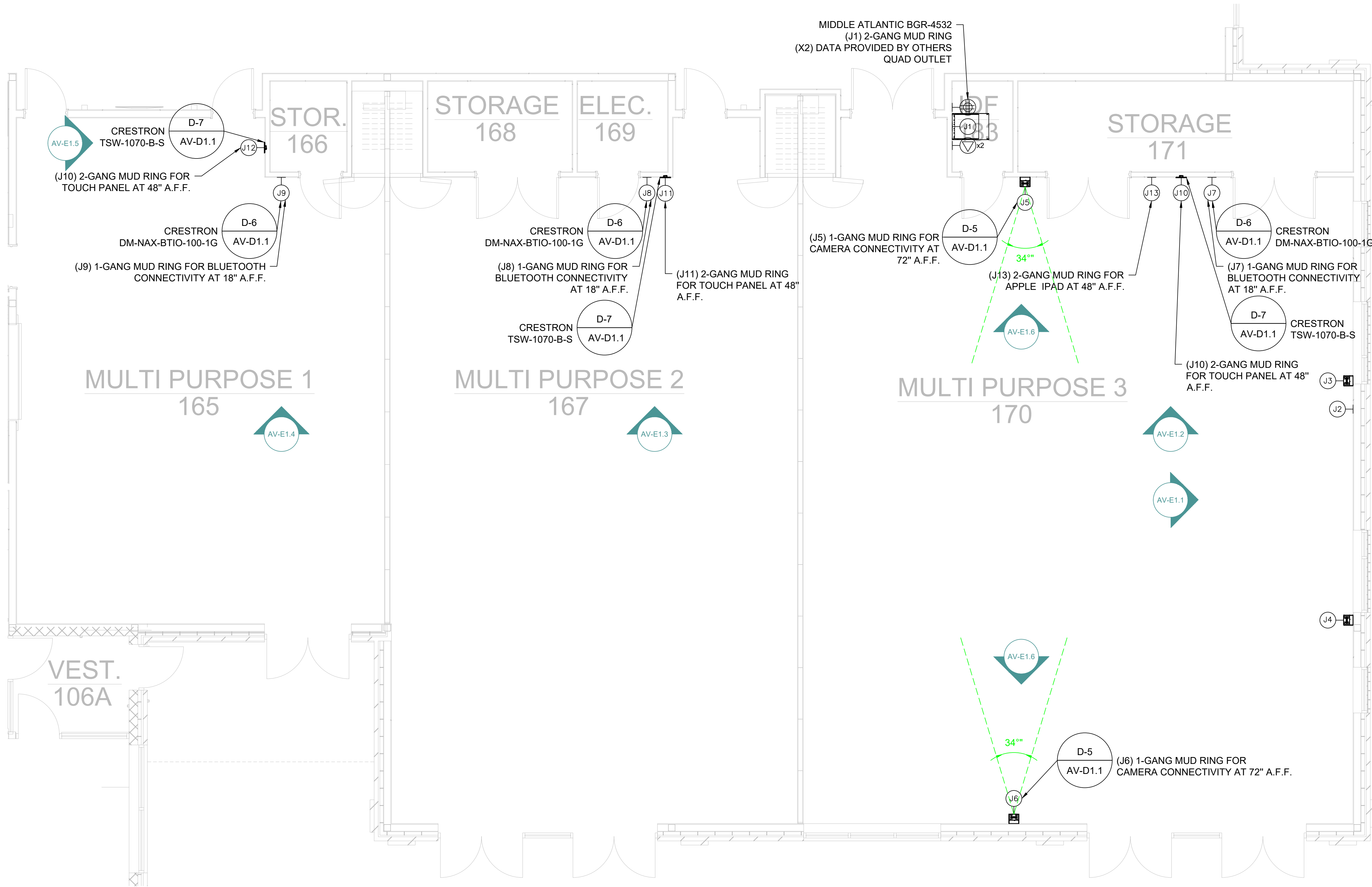
1 COMMUNITY CENTER - FLOOR PLAN SCALE: 1/4"=1'-0" ARCH D
