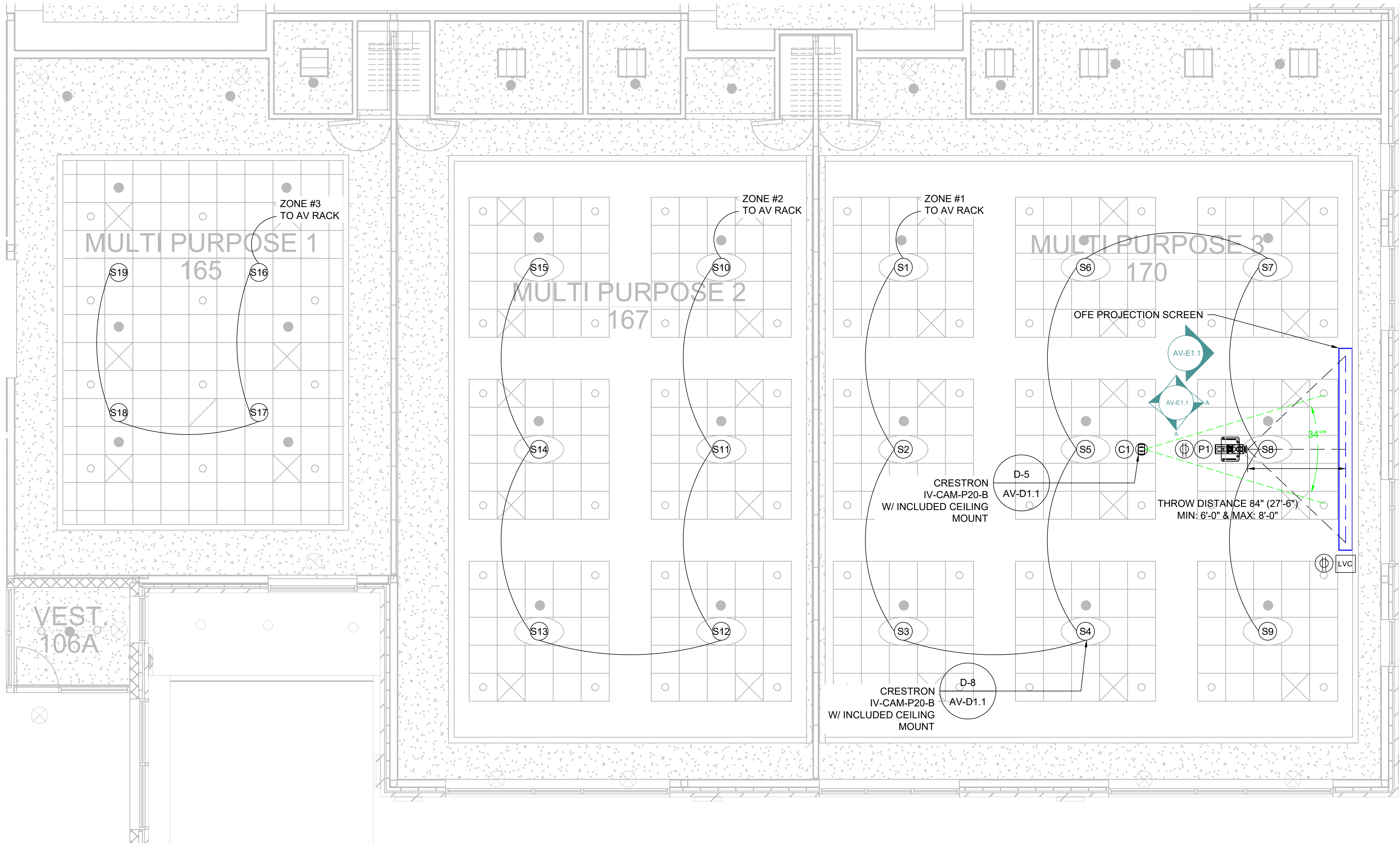
1 COMMUNITY CENTER - CEILING PLAN SCALE: 1/4"=1'-0" ARCH D
